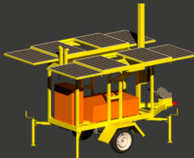
WHEEL MOBILE TOWER 800 WP
